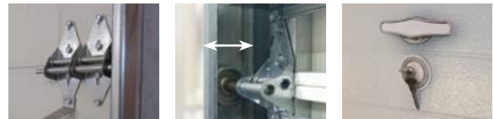
Double-end hinge
